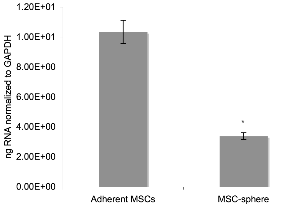
Figure 3.15: MSC-spheres significantly downregulate β-actin compared to the pre-sphere MSCs. Quantitative RT-PCR for β-actin was performed and normalized to the expression of GAPDH. (n=5 each condition; p=5.88 \times 10^{-5} paired students t-test)
